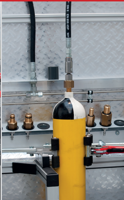
PRESSURE TEST
